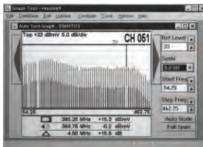
The detailed scan graph offers user-adjustable marker, scale reference level and tilt for maximum signal evaluation
